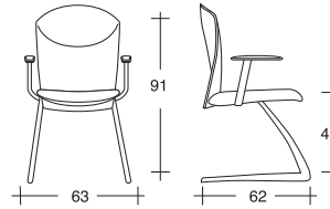
VULCAN 1495/Z
