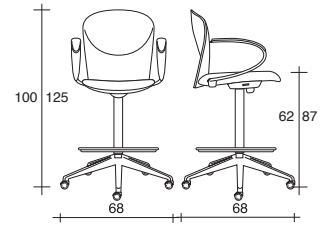
VULCAN 1336/Z
